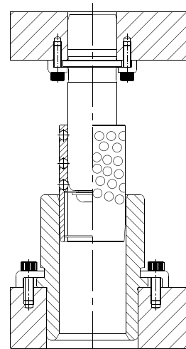
TYPE 2 PRE-LOAD RELIEVED
