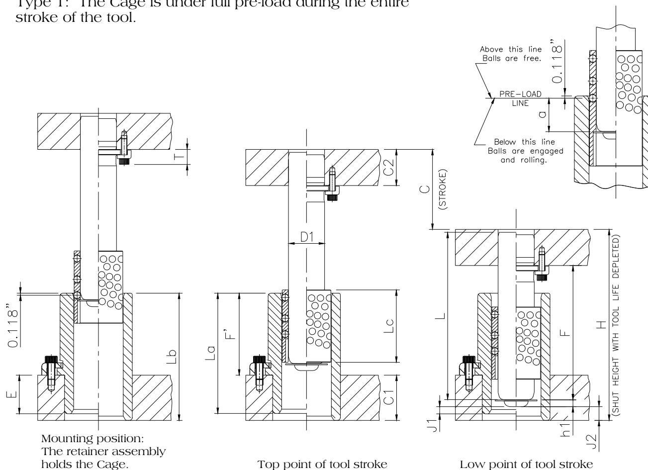
Calculations for Guide Post Length (L for Straight, F for Demountable)
